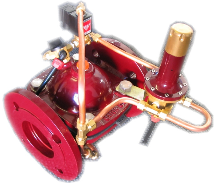
Basic Valve with Manual Override, Universal Pilots fitted for reducing operation, 3 way
