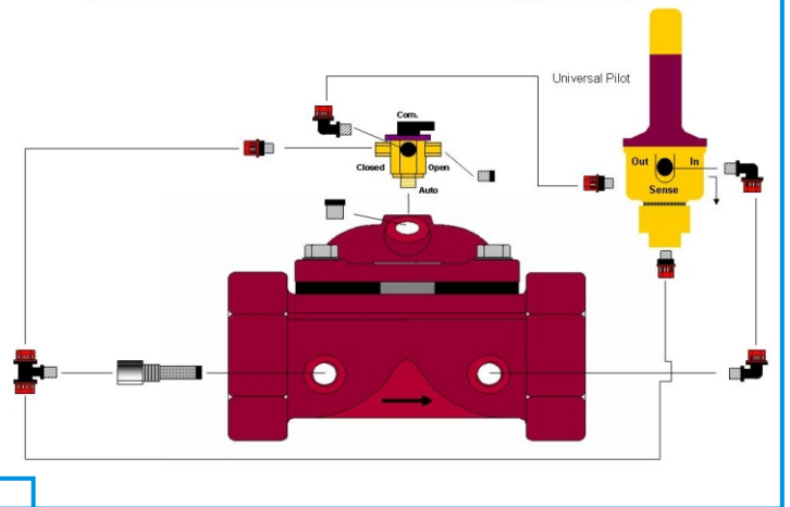
Basic Valve with Manual Override, Universal Pilots fitted for reducing operation, 3 way
