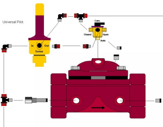
Basic Valve with Manual Override, Universal Pilots fitted for sustaining or relief operation, 3 way
